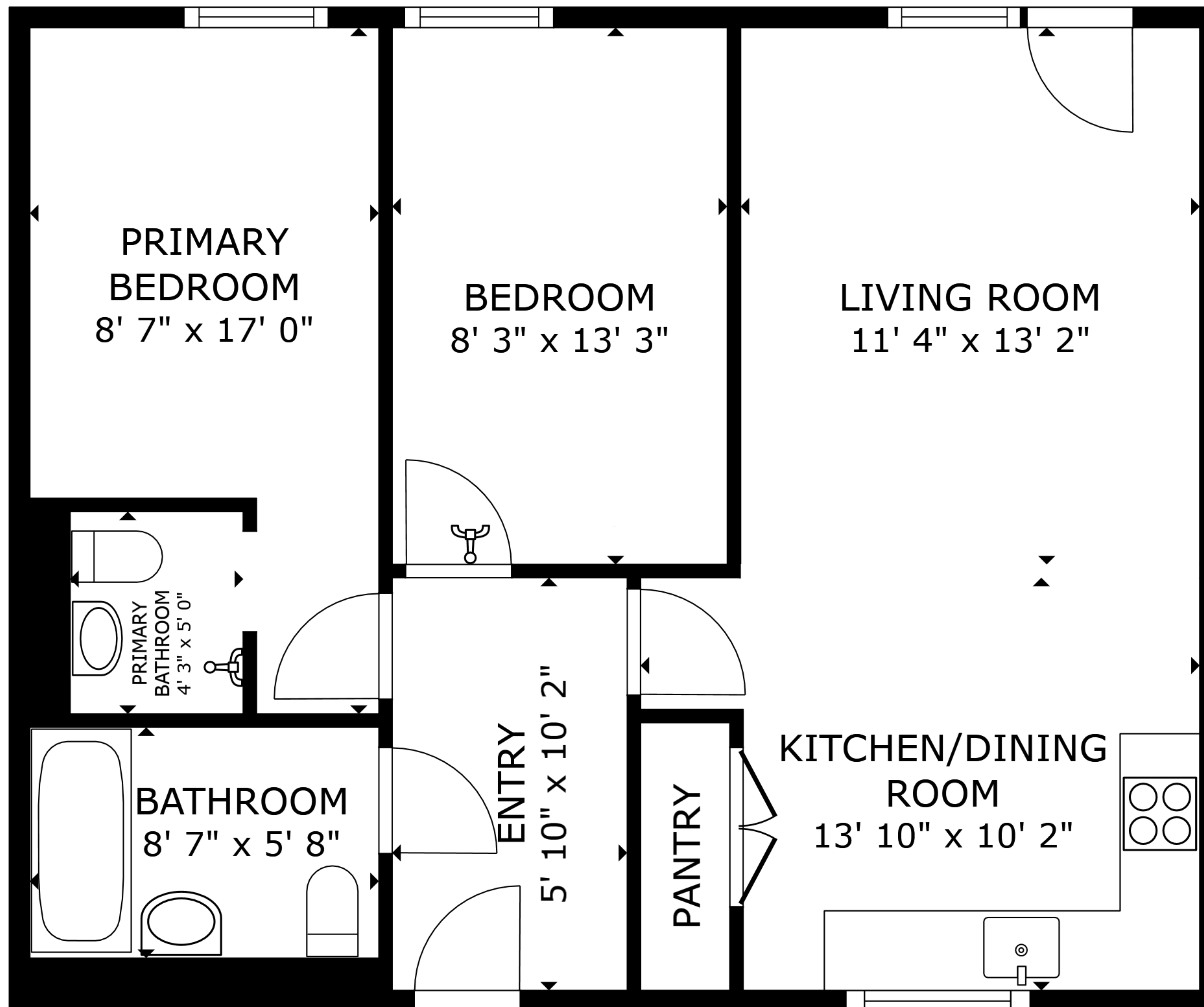
FLOOR PLAN
