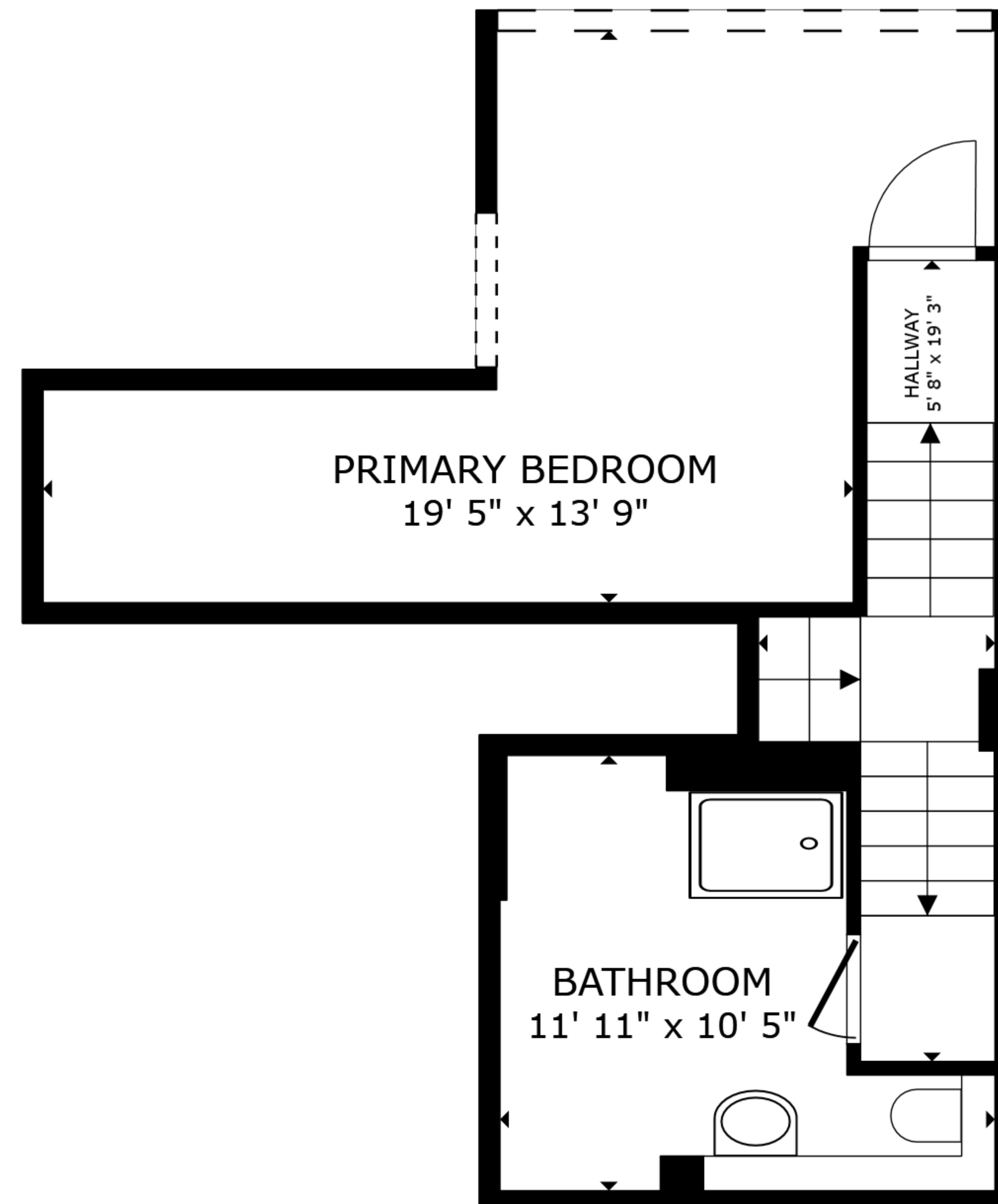
FLOOR 2
