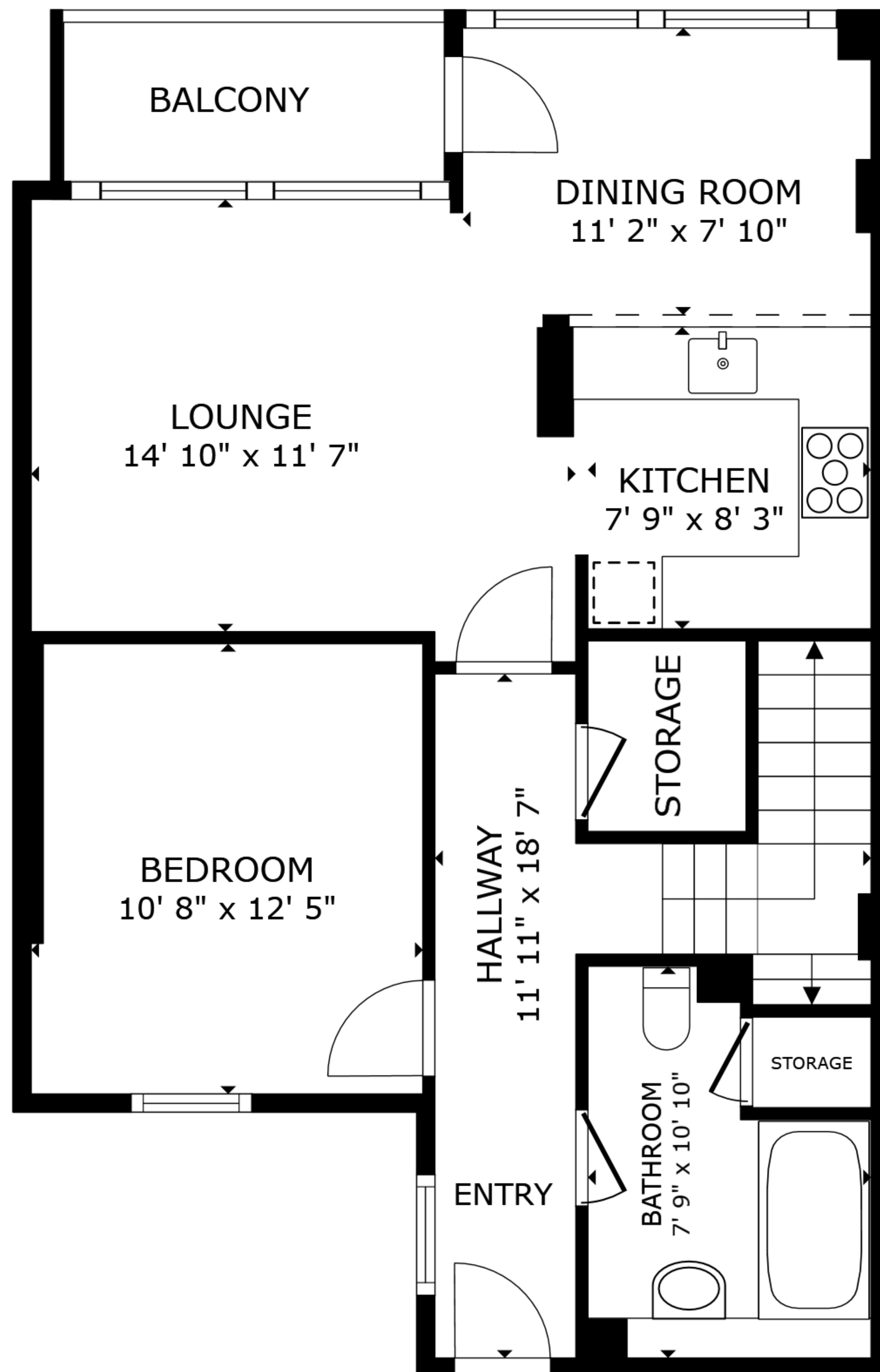
FLOOR 1
