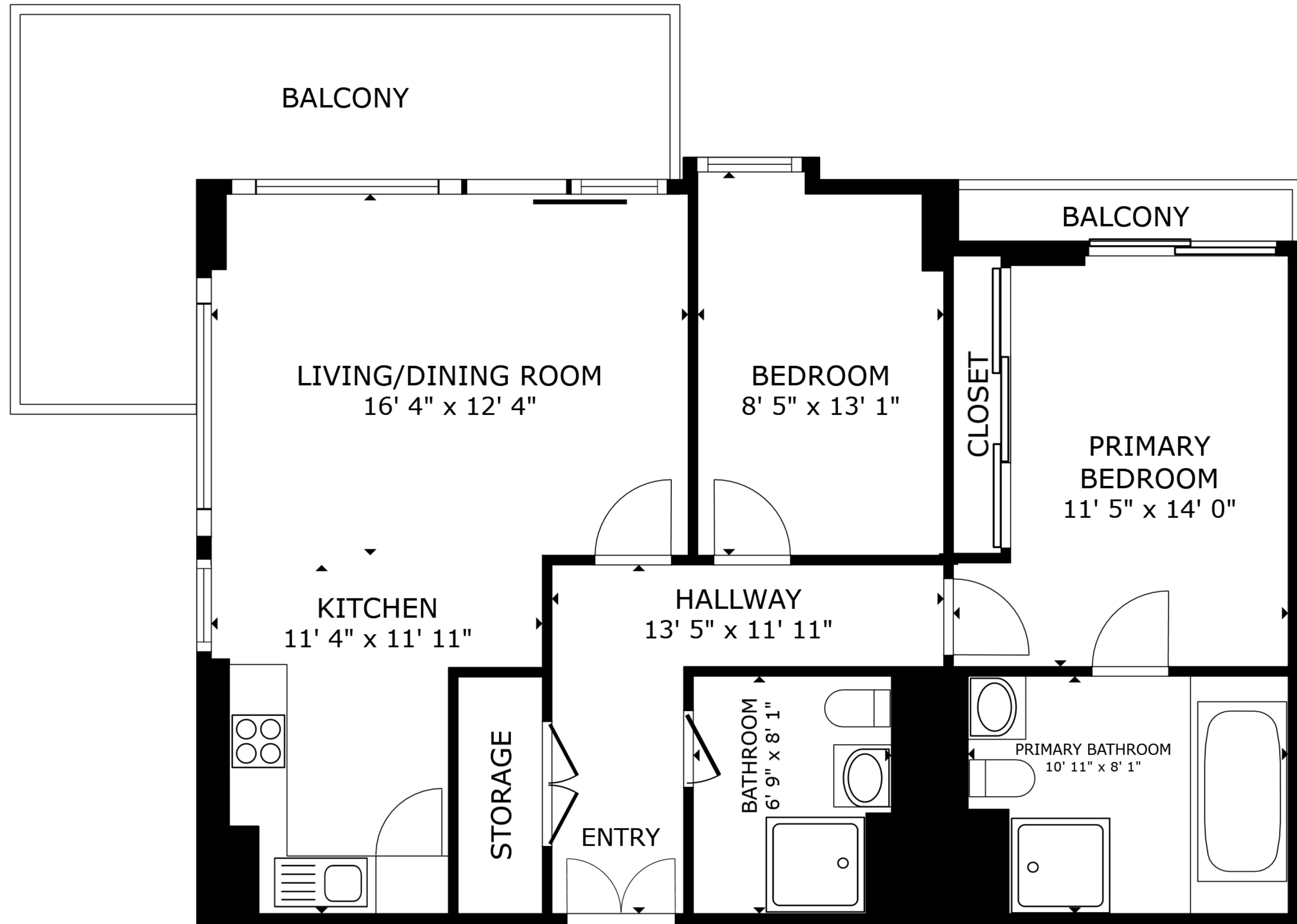
FLOOR PLAN
