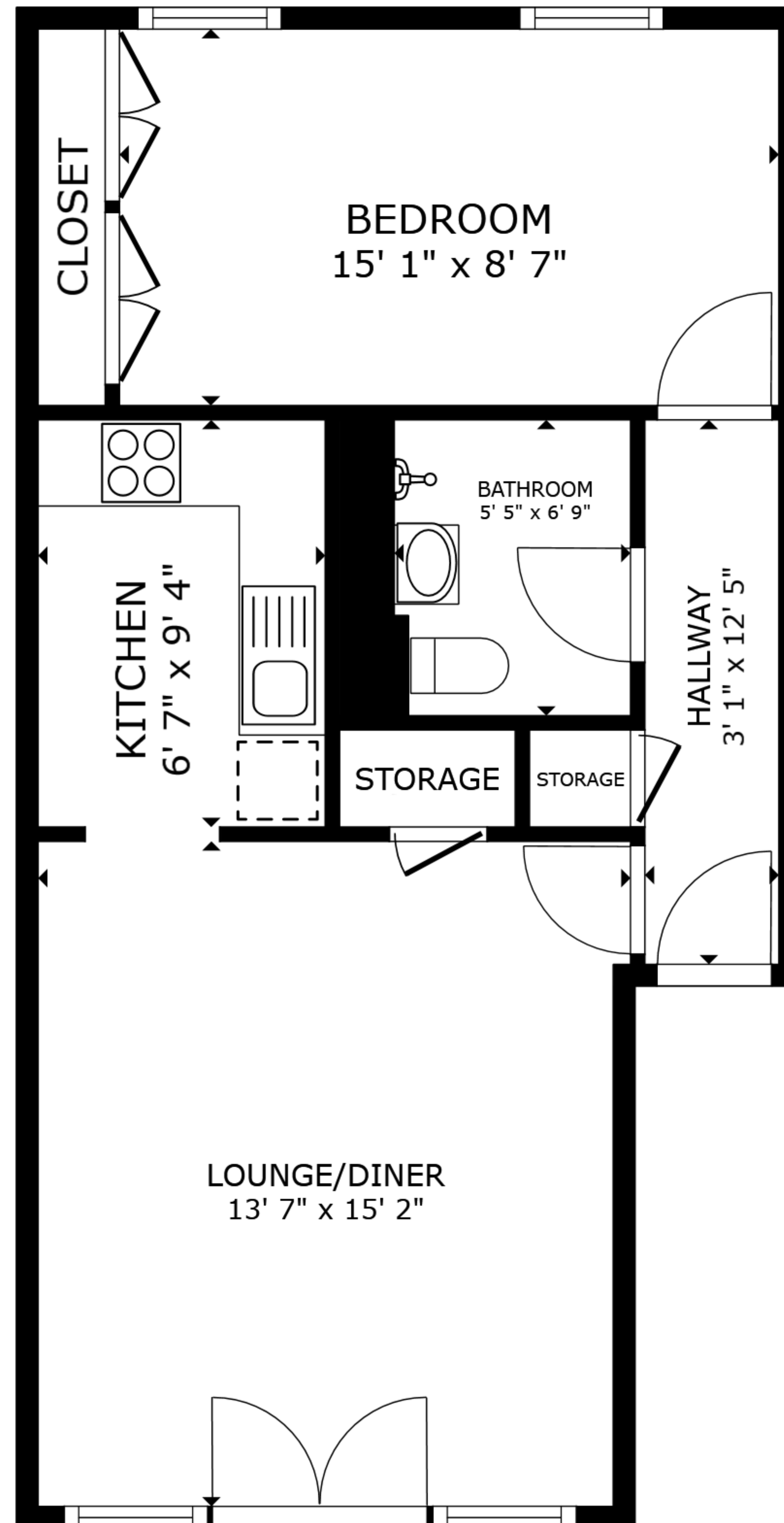
FLOOR PLAN
