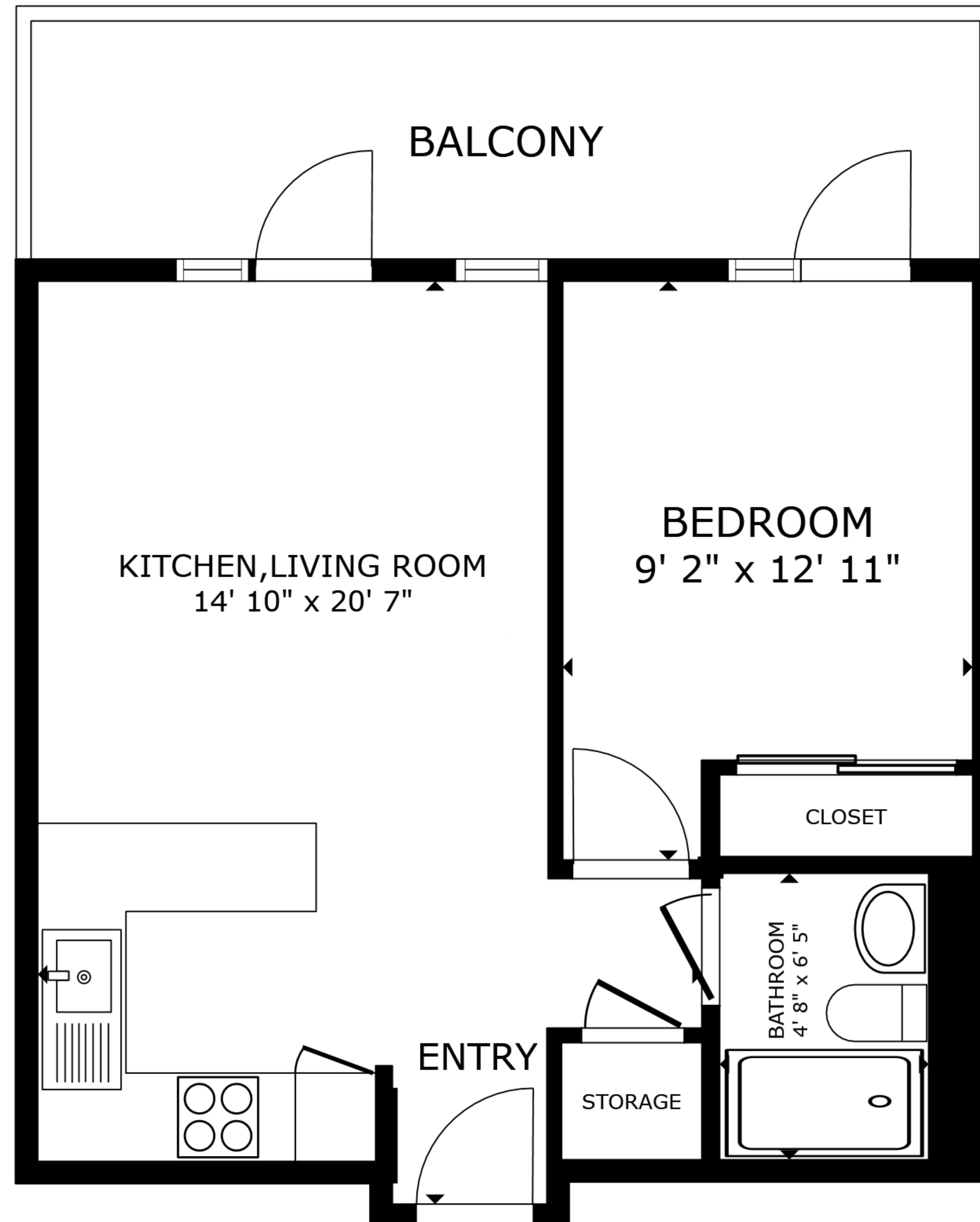
FLOOR PLAN
