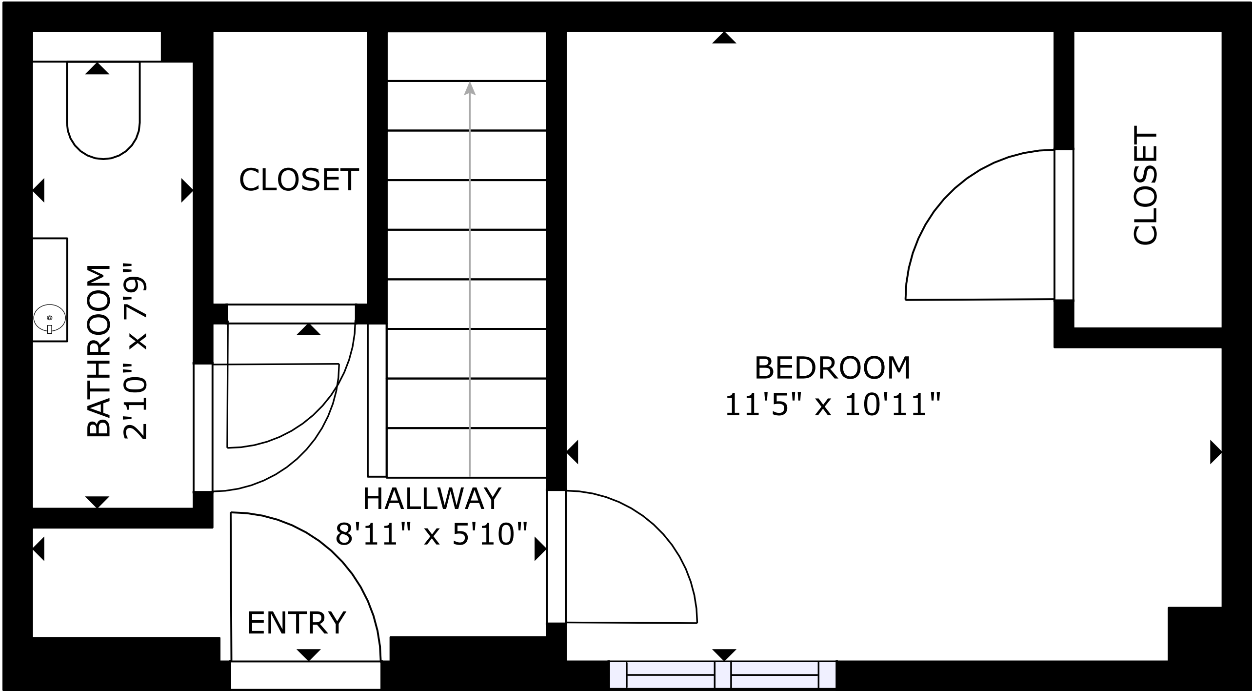
FLOOR 1
