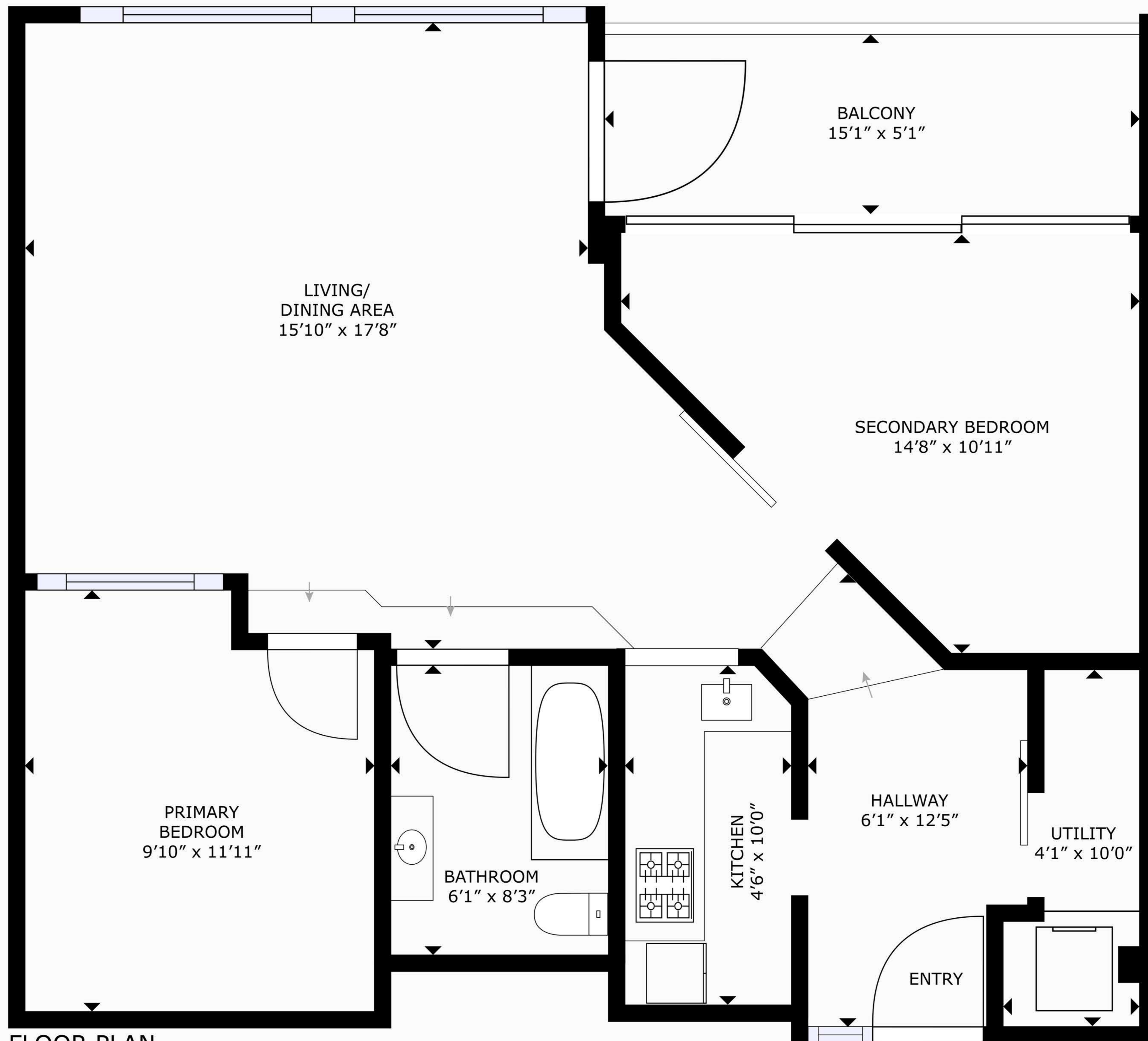
FLOOR PLAN
