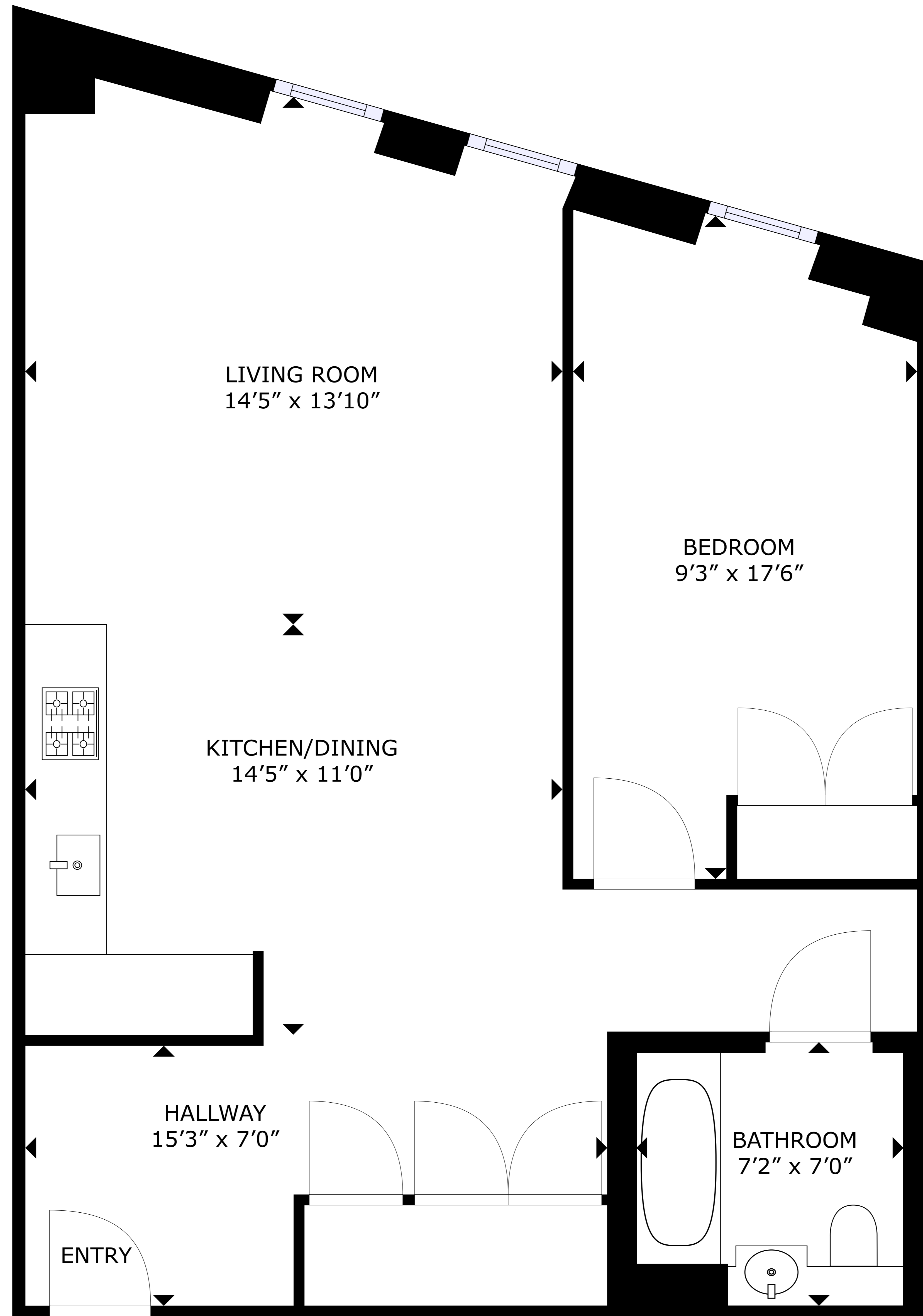
FLOOR PLAN
